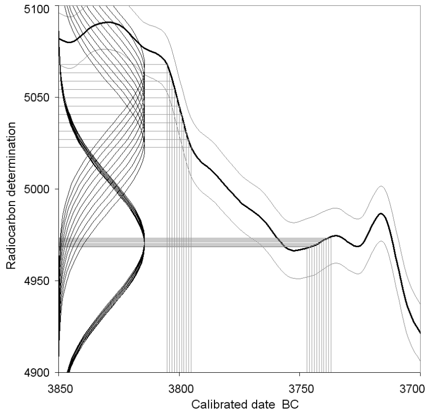
Figure 2 For each calendar year, the responding 14 C age is calculated and the Gaussian curve is obtained. All Gausses are totaled with the weight depending on calendar age (see Figure 1). Finally, the median of the sum is calculated. Only 2 groups of "samples" are presented for clarity (taken for extreme calibration curve slopes).
