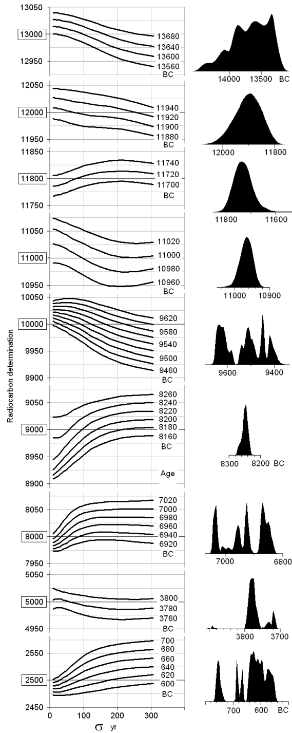
Figure 3 The 14 C (median) age as a function of the measurement error \sigma , for different calendar (BC) ages of the trial “center” of the large group of samples. Because lines are not strictly horizontal, the “calibration” of Mangerud’s boundaries, in some cases only, is almost independent of \sigma . (The “conventional” description of the vertical axis is somehow incorrect here due to the different meanings of the word “determination.”) Standard calibration (OxCal 4.1) of discussed boundaries, obtained with \sigma = 0 , is given for comparison purposes.
